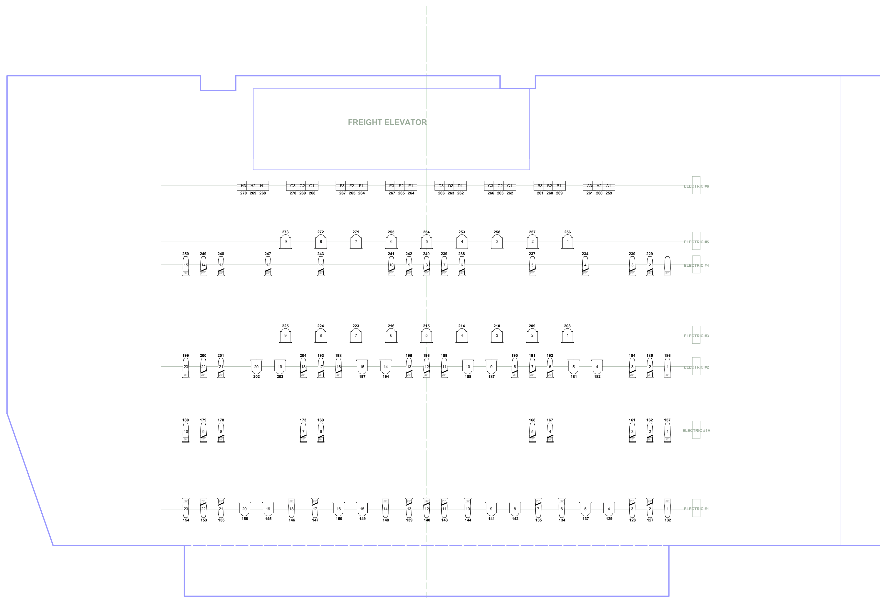
OHIO THEATRE LIGHT PLOT Scale: 1/4" = 1'-0"
